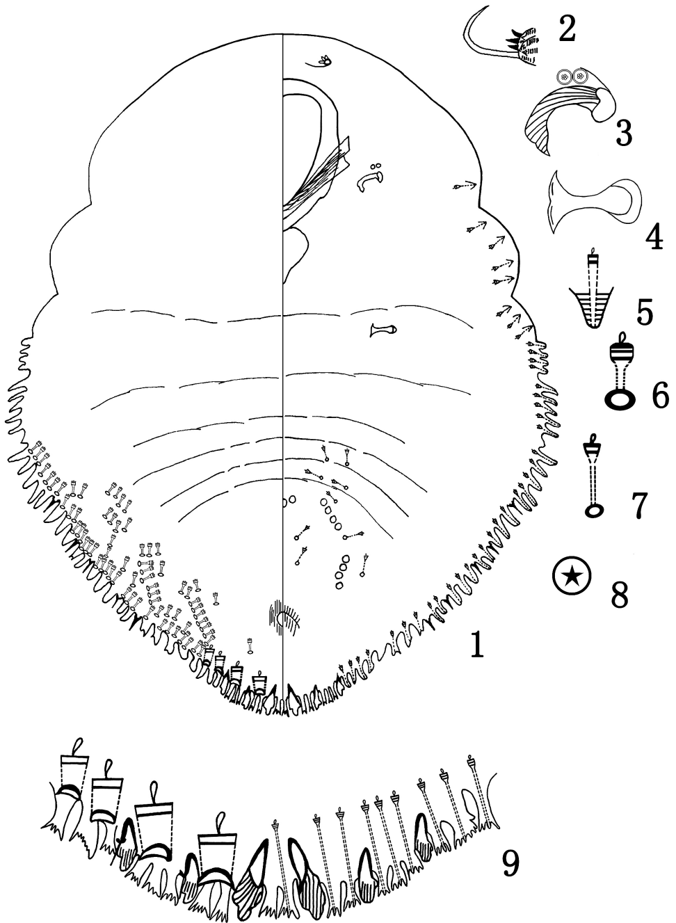
Figure 1–9. Parlatoria menglaensis sp. n., adult female. 1 body 2 antenna 3 anterior spiracle 4 posterior spiracle 5 gland tubercle 6 detail of dorsal gland duct 7 ventral microduct 8 perivulvar pore 9 pygidium.
