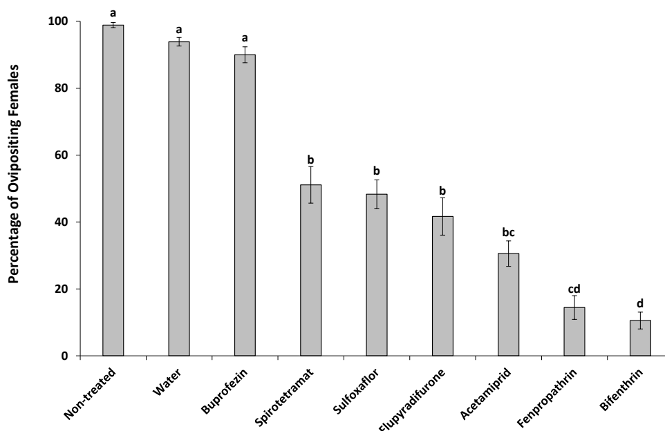
Figure 4. The relationship between different treatments and the percentage of adult females of Maconellicoccus hirsutus with successful oviposition (ANOVA summary: F_{8,98} = 76.58 , p < 0.001 ). Bars with the same letter are not significantly different (Games-Howell Test, p < 0.05 ).
